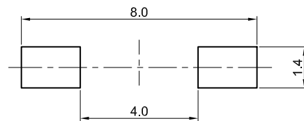
PRINTED CIRCUIT BOARD DIMENSIONS (WHEN VIEWED FROM SWITCH MOUNTING FACE)
