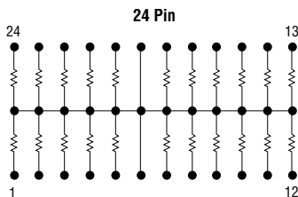
GTL (Gunning Transceiver Logic) Termination Network
