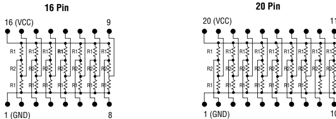
Differential Ended SCSI (Small Computer System Interface) Termination Network
