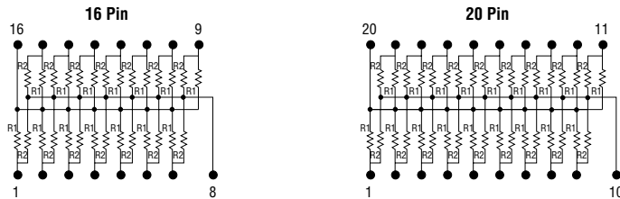
Single Ended SCSI (Small Computer System Interface) Termination Network
